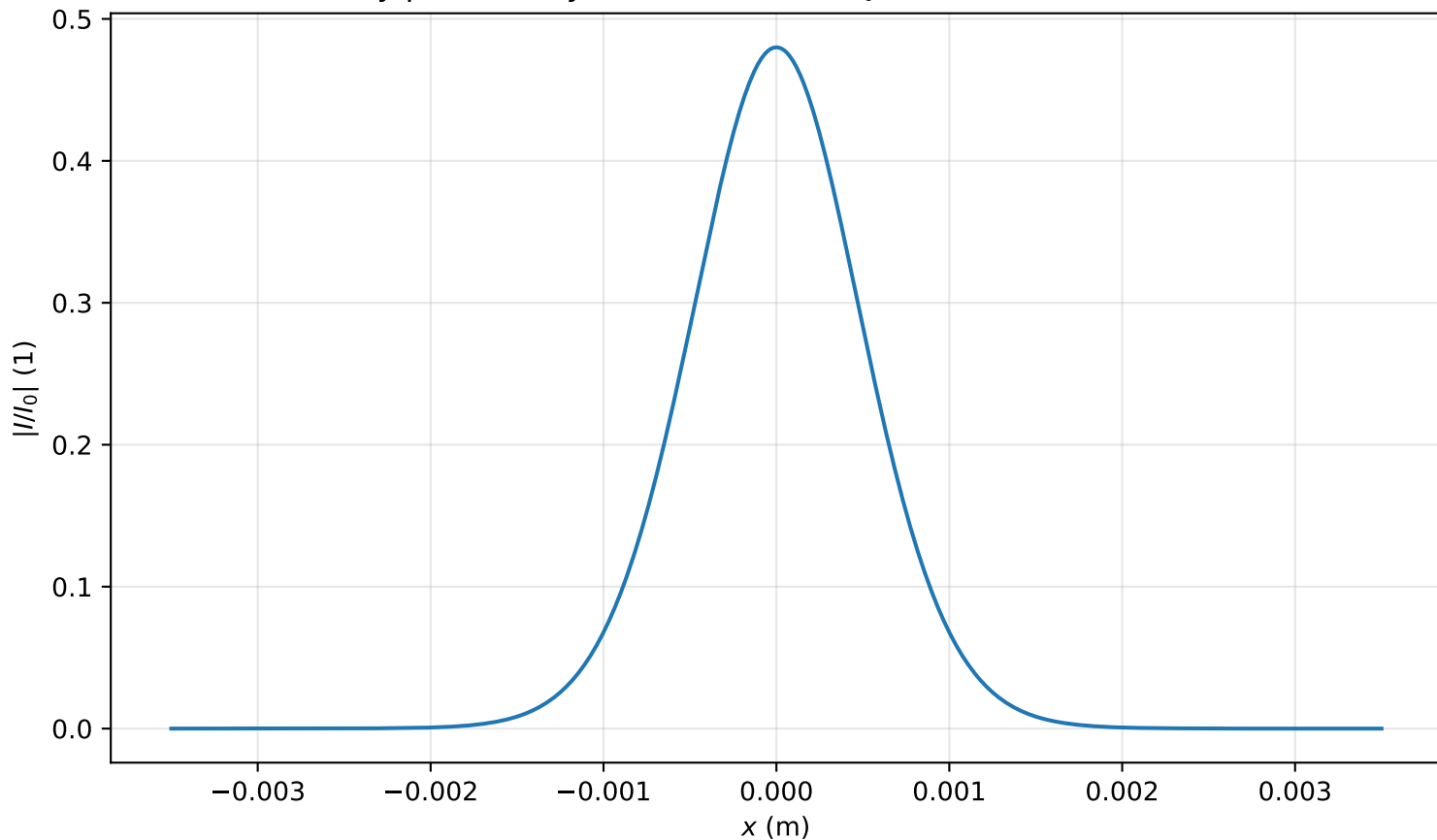
Intensity profile I(x, y = 0, z = 2.707m)/I_0 , P_{in}=0.3P_{cr} , artificial time
